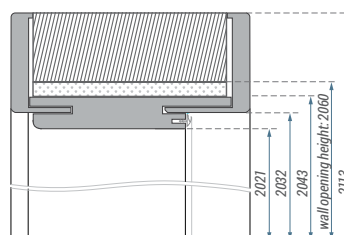
▼ ADJUSTABLE DOOR FRAME NON-REBATED 80
